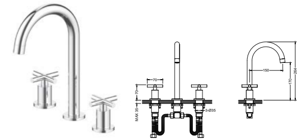
AT090214 3-hole basin mixer /Finish: CH /BN /MB /BG /RG /BGM
