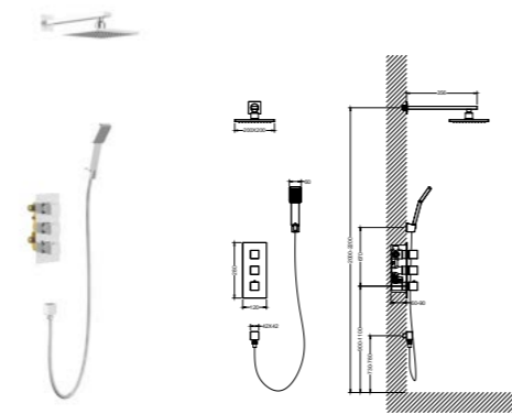
AT083201 Shower Mixer Set /Finish: CH /BN /MB
