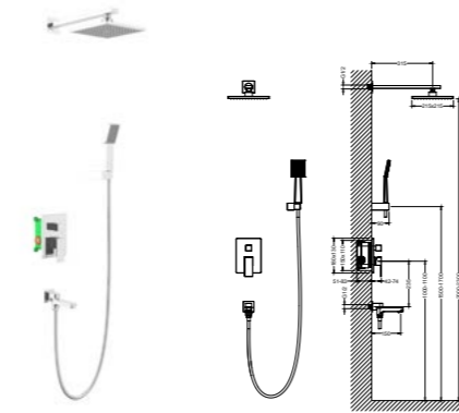
AT082202 Shower Mixer Set /Finish: CH /BN /MB
