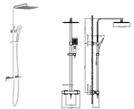
AT080072 2 ways thermostatic shower column /Finish: CH /BN /MB
