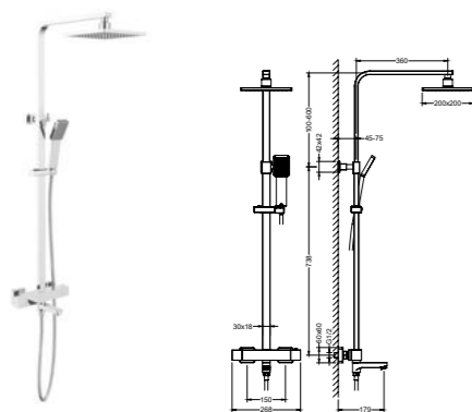
AT080075 3 ways thermostatic shower column /Finish: CH /BN /MB
