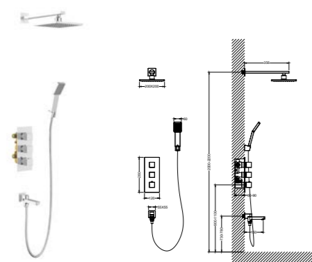
AT083202 Shower Mixer Set /Finish: CH /BN /MB
