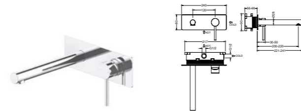
AT090216 Concealed basin mixer with W-BOX /Finish: CH /BN /MB /BG /RG /BGM
