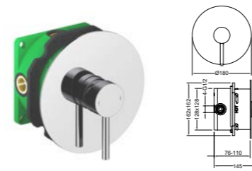
AT090151 Concealed shower mixer with W-BOX /Finish: CH /BN /MB /BG /RG /BGM
