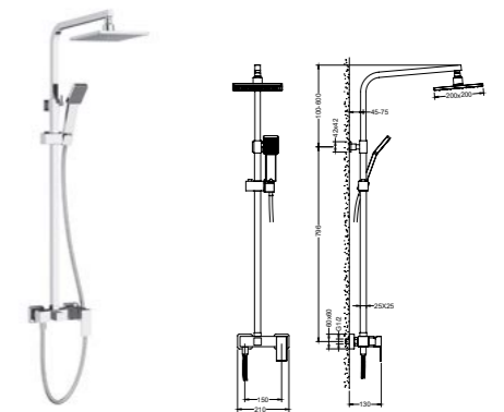
AT080065 2 ways shower column /Finish: CH /BN /MB
