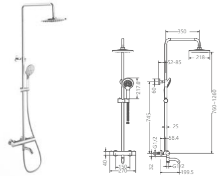
TWL1119-01 Thermostatic three function shower /Finish: CH
