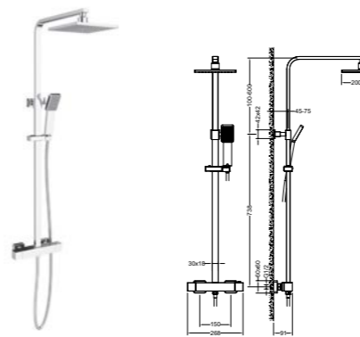
AT080071 2 ways thermostatic shower column /Finish: CH /BN /MB
