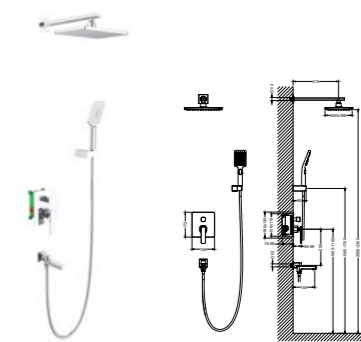
AT212203 3 ways shower column /Finish: CH /BN /MB /CH+White
