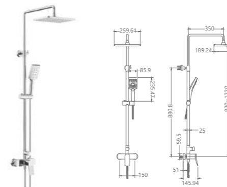
TWL1154-01 Single function shower /Finish: CH /MB
