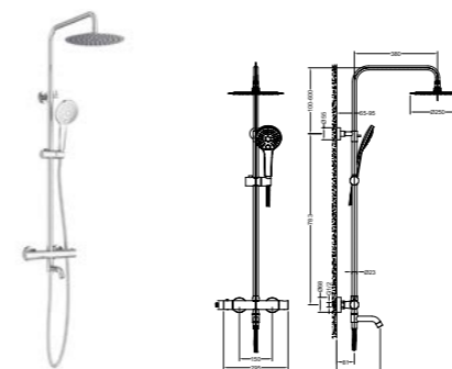
AT090074 3 ways shower mixer set /Finish: CH /BN /MB /BG /RG /BGM
