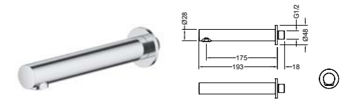
AT090254 Concealed basin mixer with W-BOX /Finish: CH /BN /MB /BG /RG /BGM
