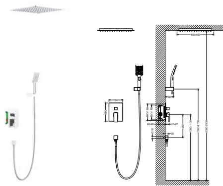
AT082203 Shower Mixer Set /Finish: CH /BN /MB
