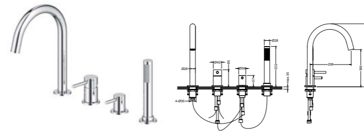
AT090025 Bath mixer /Finish: CH /BN /MB /BG /RG /BGM
