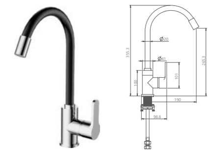
TWP0249-08 Kitchen faucet /Finish: CH
