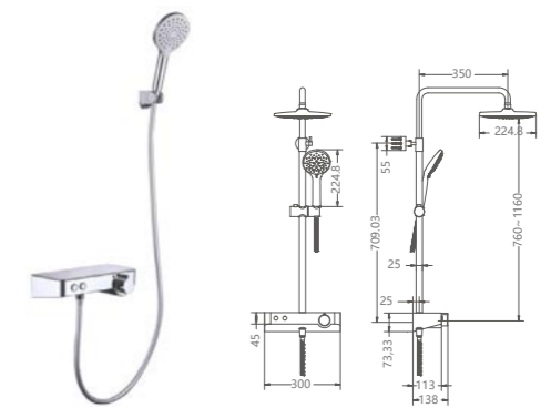
TWL1139-01 Two function shower /Finish: CH /MB
