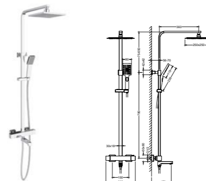
AT080073 3 ways thermostatic shower column /Finish: CH /BN /MB
