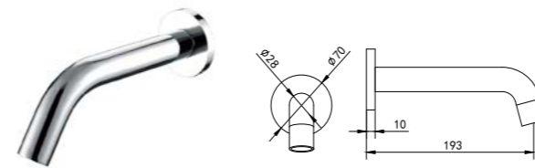
TWY0013-01 Sensor faucet /Finish: CH
