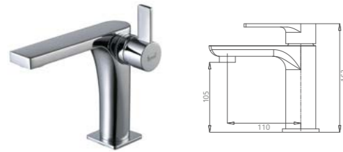
TWG0544-01 Basin mixer /Material: Brass
