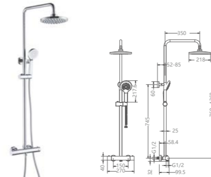
TWL0663-01 Thermostatic two function shower /Finish: CH
