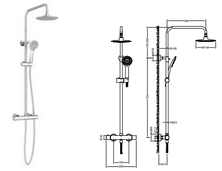
AT090071 2 ways shower mixer set /Finish: CH /BN /MB /BG /RG /BGM
