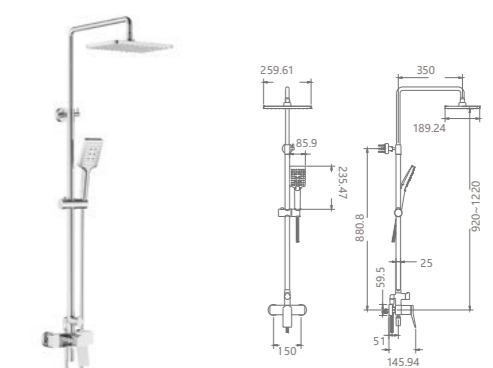
TWL1155-01 Single function shower /Finish: CH /MB
