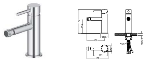
AT090231 Wall-in tap /Finish: CH /BN /MB /BG /RG /BGM
