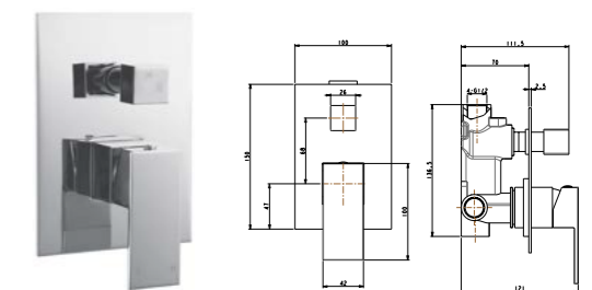
AY34B18YC WaterMark Wall Shower /Bath Mixer With Diverter /Finish: CH /MB
