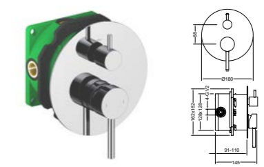
AT090152 Concealed bath shower mixer with W-BOX /Finish: CH /BN /MB /BG /RG /BGM
