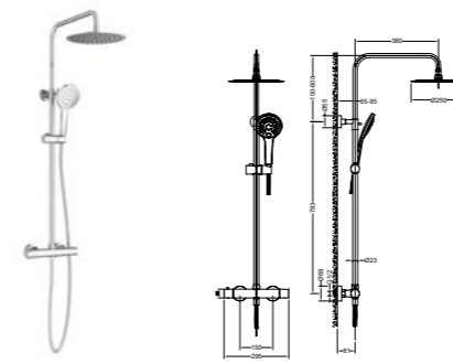
AT090072 2 ways shower mixer set /Finish: CH /BN /MB /BG /RG /BGM
