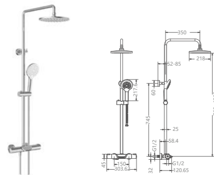
TWL1138-01 Thermostatic three function shower /Finish: CH /MB
