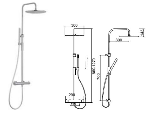
TWL1117-01 Two function shower /Finish: CH
