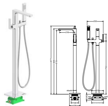
AT210128 Floor standing bath shower mixer /Finish: CH /BN /MB /CH+White
