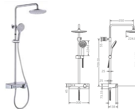
TWL1140-01 Two function shower /Finish: CH /MB
