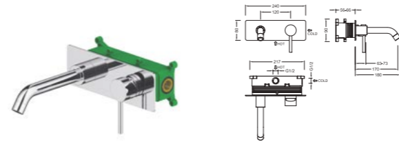
AT090117 Concealed basin mixer with W-BOX /Finish: CH /BN /MB /BG /RG /BGM
