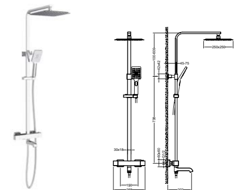
AT080074 3 ways thermostatic shower column /Finish: CH /BN /MB
