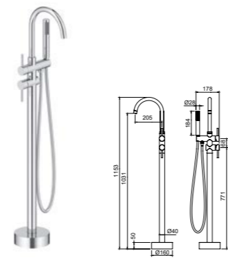
AT090029 Floor standing bath shower mixer /Finish: CH /BN /MB /BG /RG /BGM
