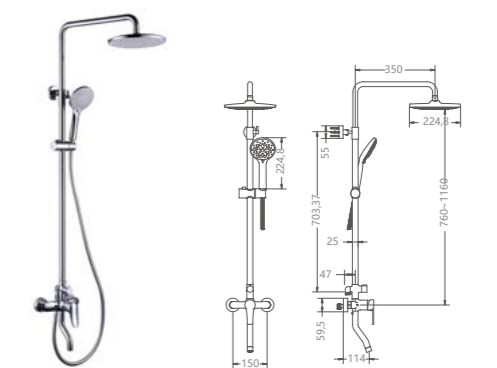
TWL1142-01 Three function shower /Finish: CH /MB
