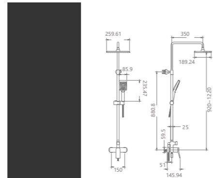
TWL1155-01 Single function shower /Finish: CH /MB
