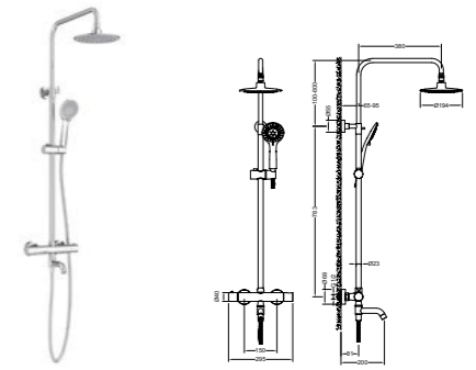
AT090073 3 ways shower mixer set /Finish: CH /BN /MB /BG /RG /BGM
