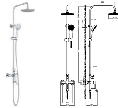
AT090061 3 ways shower mixer set /Finish: CH /BN /MB /BG /RG /BGM
