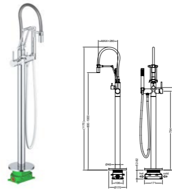
AT090129 Floor standing bath shower mixer /Finish: CH /BN /MB /BG /RG /BGM
