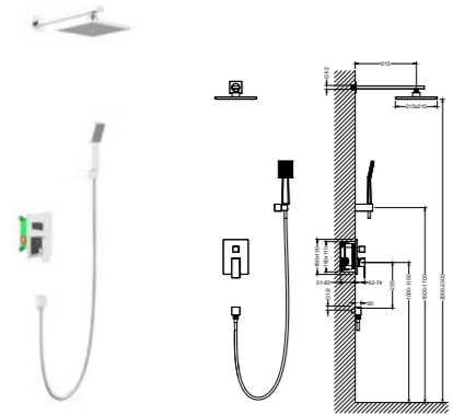
AT082201 Shower Mixer Set /Finish: CH /BN /MB
