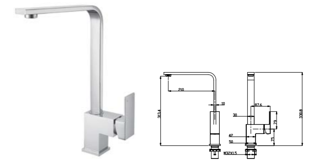
AY56B18YC WaterMark Kitchen Mixer /Finish: CH /MB
