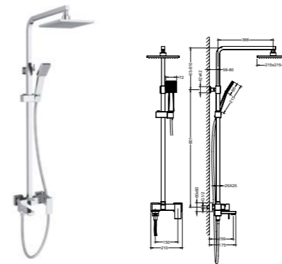
AT080064 3 ways shower column /Finish: CH /BN /MB
