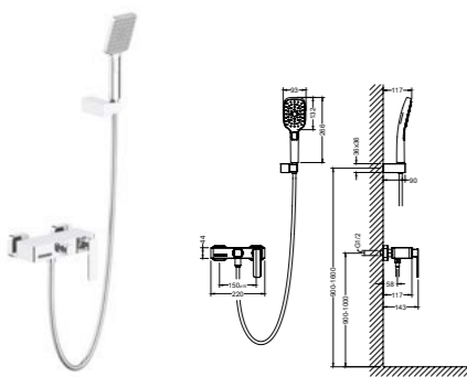
AT210122 Basin mixer /Finish: CH /BN /MB /CH+White
