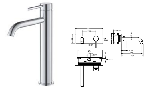
AT090112 Single lever vessel basin mixer, sleek handle /Finish: CH /BN /MB /BG /RG /BGM
