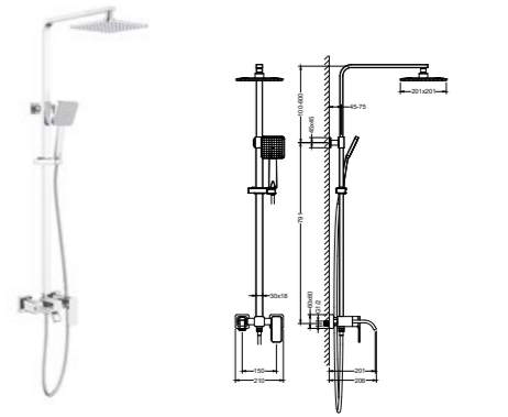
AT080067 3 ways shower column /Finish: CH /BN /MB
