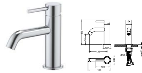
AT090011 Single lever basin mixer /Finish: CH /BN /MB /BG /RG /BGM
