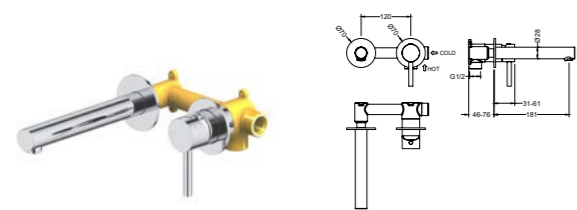
AT090215 Concealed basin mixer /Finish: CH /BN /MB /BG /RG /BGM
