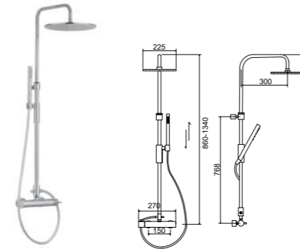
TWL1116-01 Two function shower /Finish: CH
