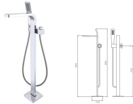
TWG0503-01 Freestanding mixer /Finish: CH
