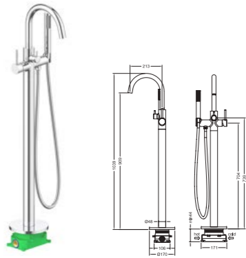
AT090128 Floor standing bath shower mixer /Finish: CH /BN /MB /BG /RG /BGM
