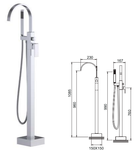
AT080029 Floor standing bath shower mixer /Finish: CH /BN /MB
