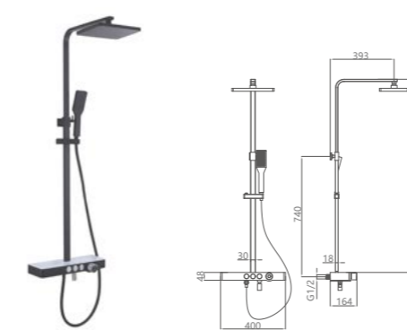
TWL6119-02 Three function shower /Finish: CH /MB
