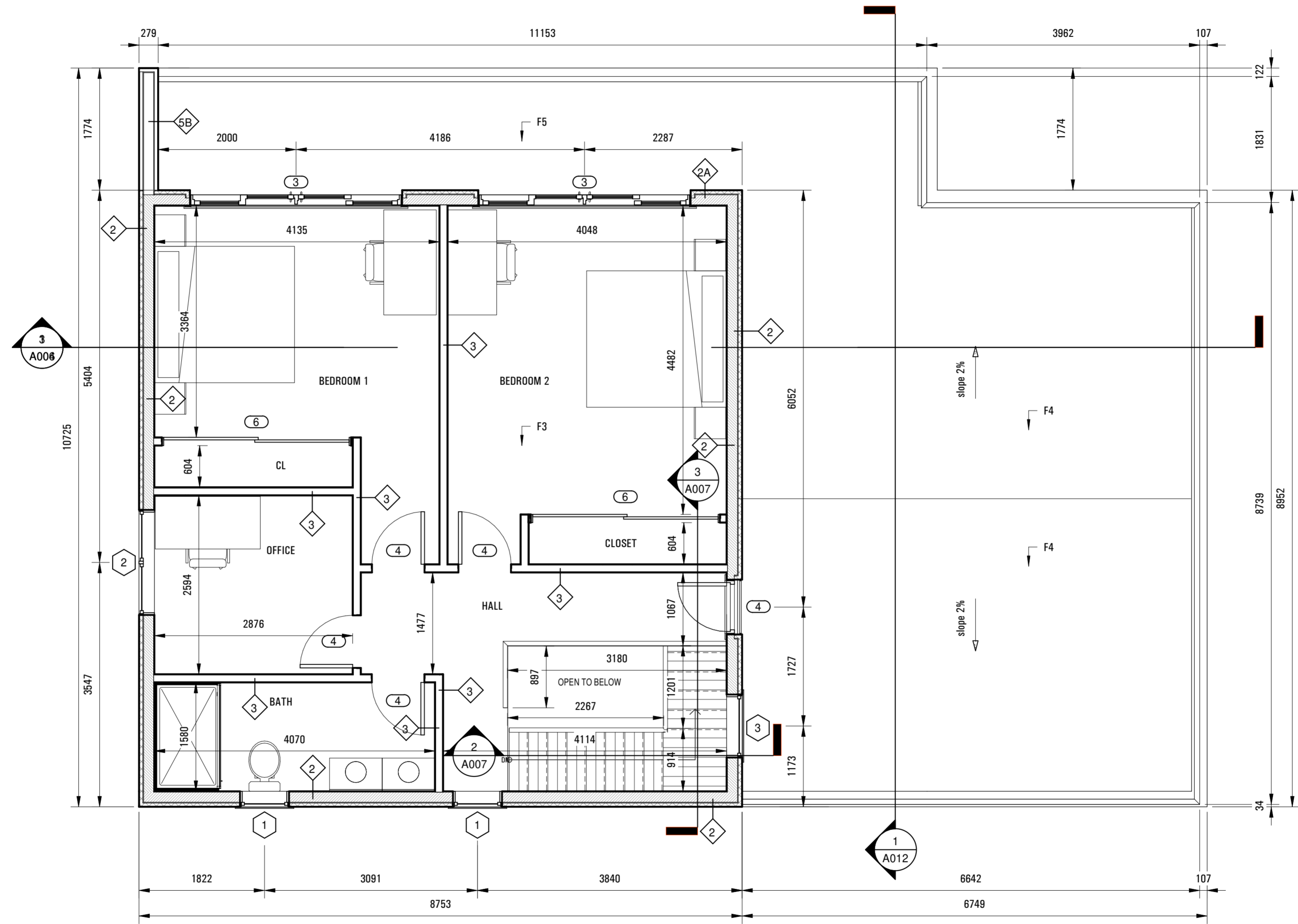
1 2ND FLOOR PLAN 1/4" = 1'-0"
