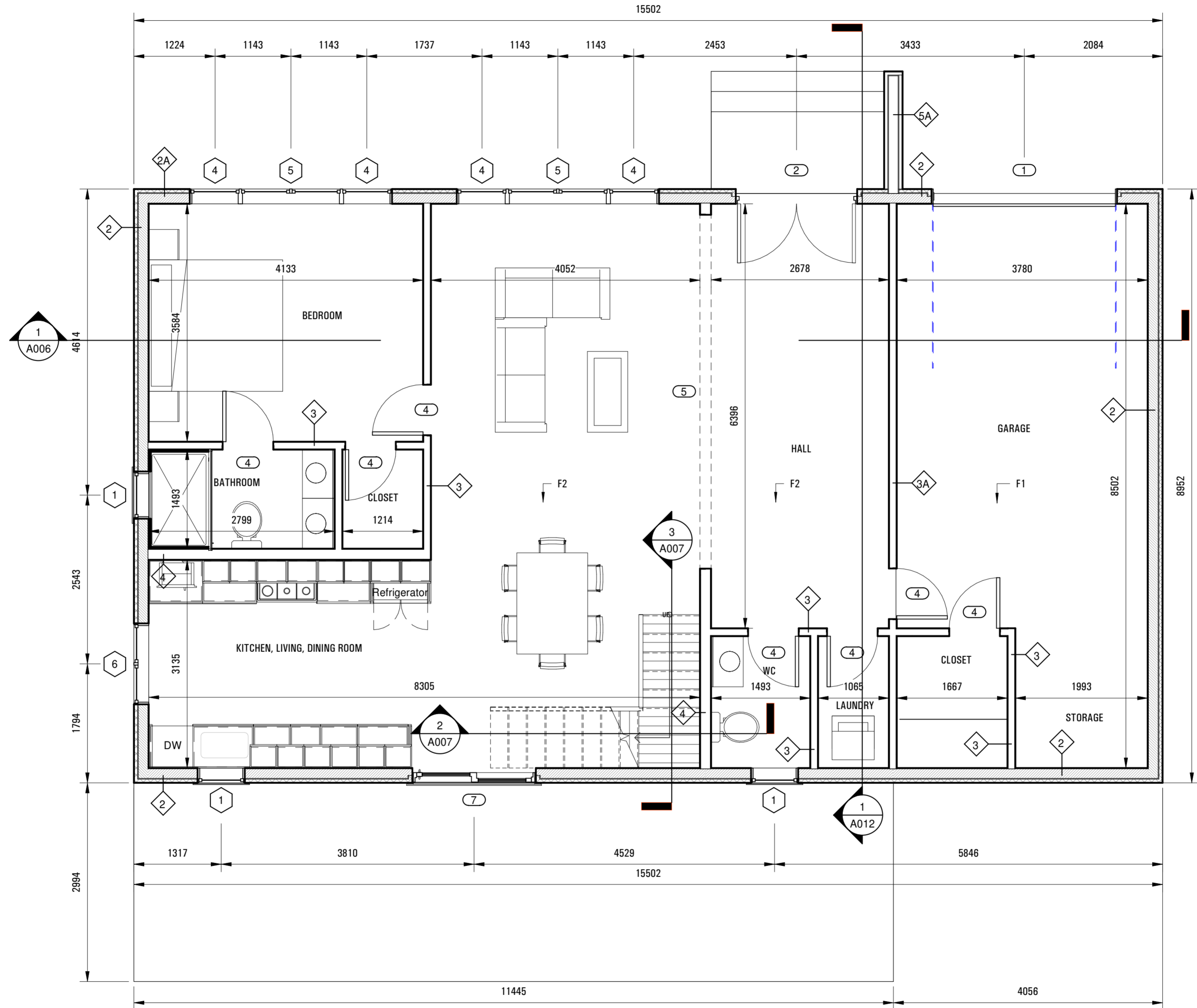
1 | 1ST FLOOR PLAN 1/4" = 1'-0"
